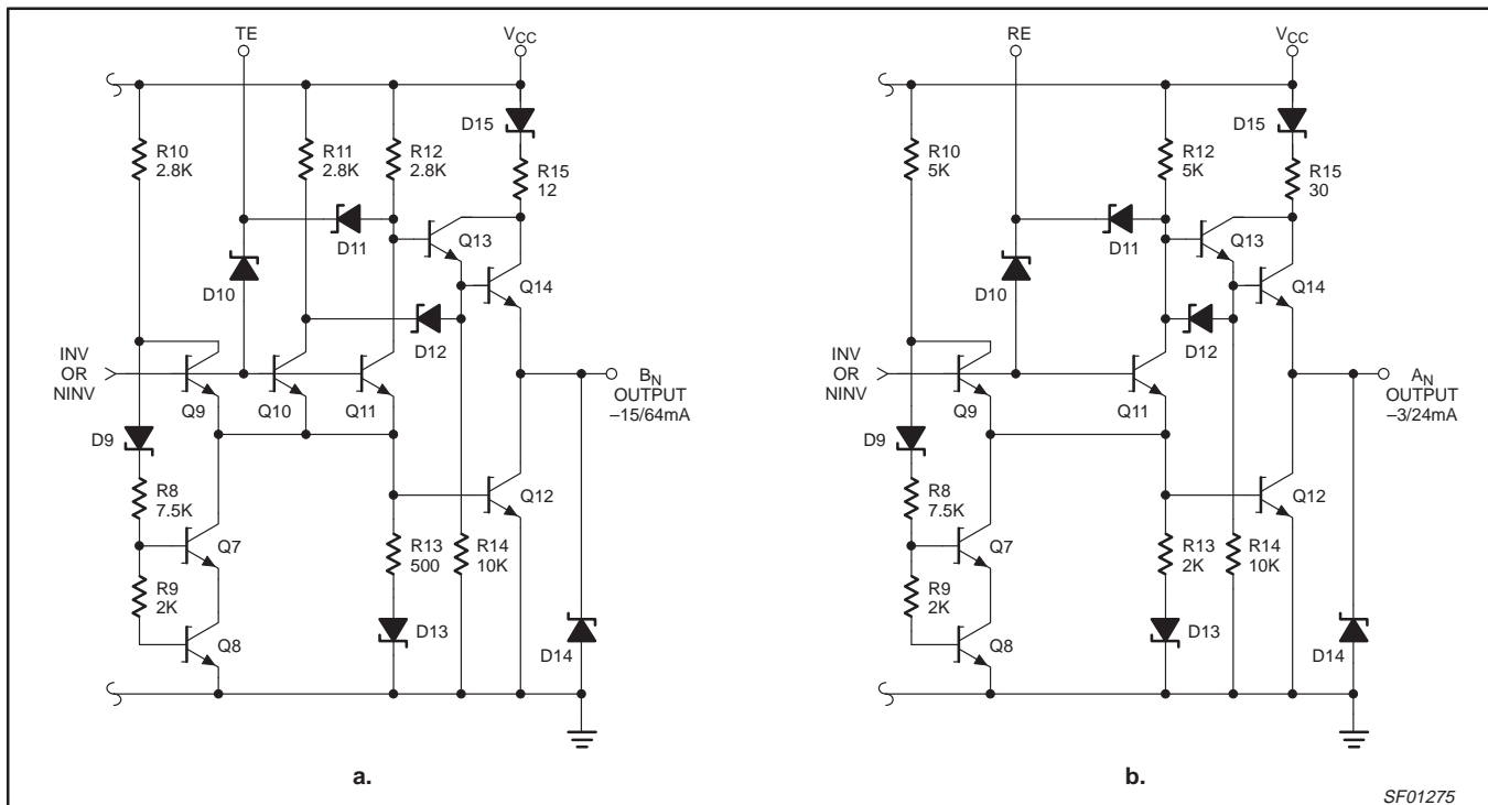
Figure 4. Two Typical "Light Load" Output Structures (74F657)
