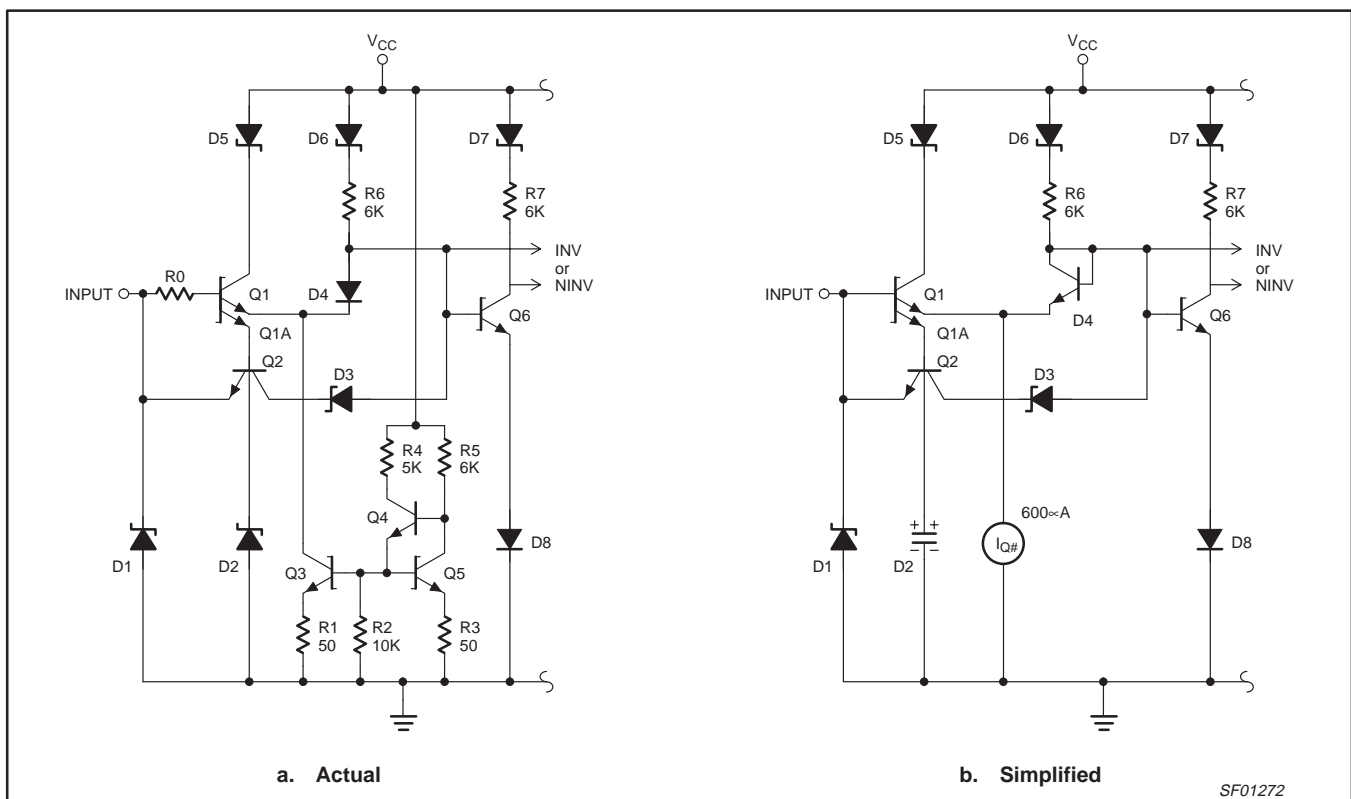
Figure 1. The "Light Load" and Speed-Up Circuit Input Structure (Actual & Simplified)
