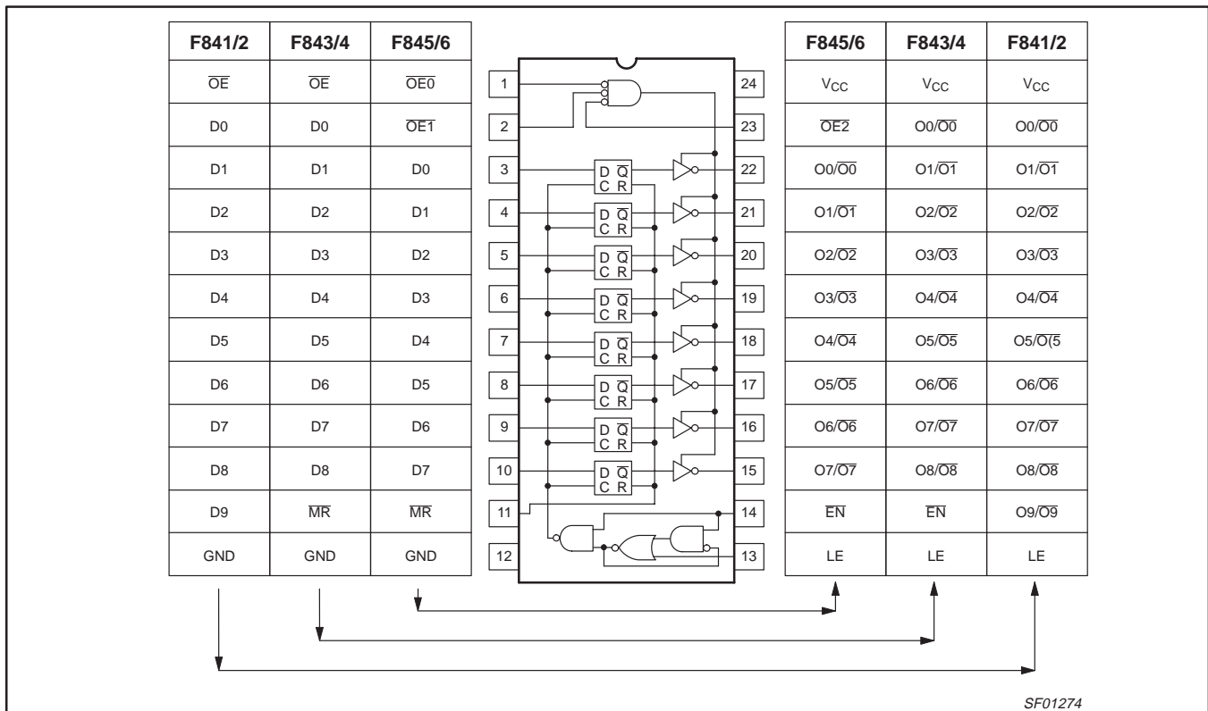
Figure 3. 74F84X Latched Buffer Pin Configurations
