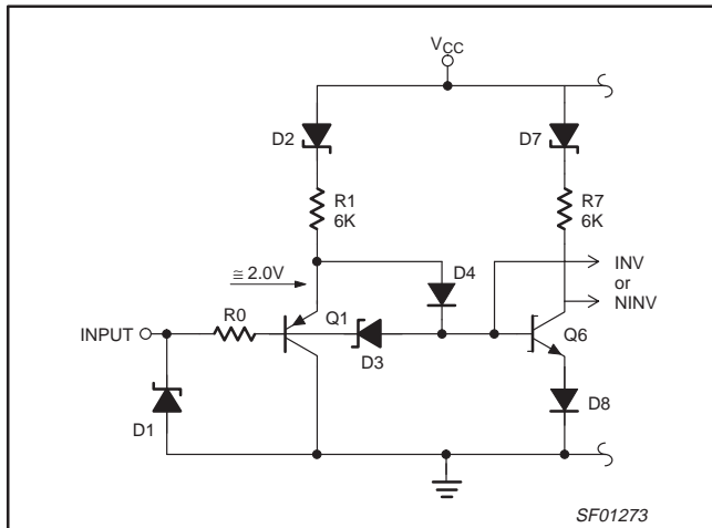
Figure 2. Future "Light Load" PNP Input
