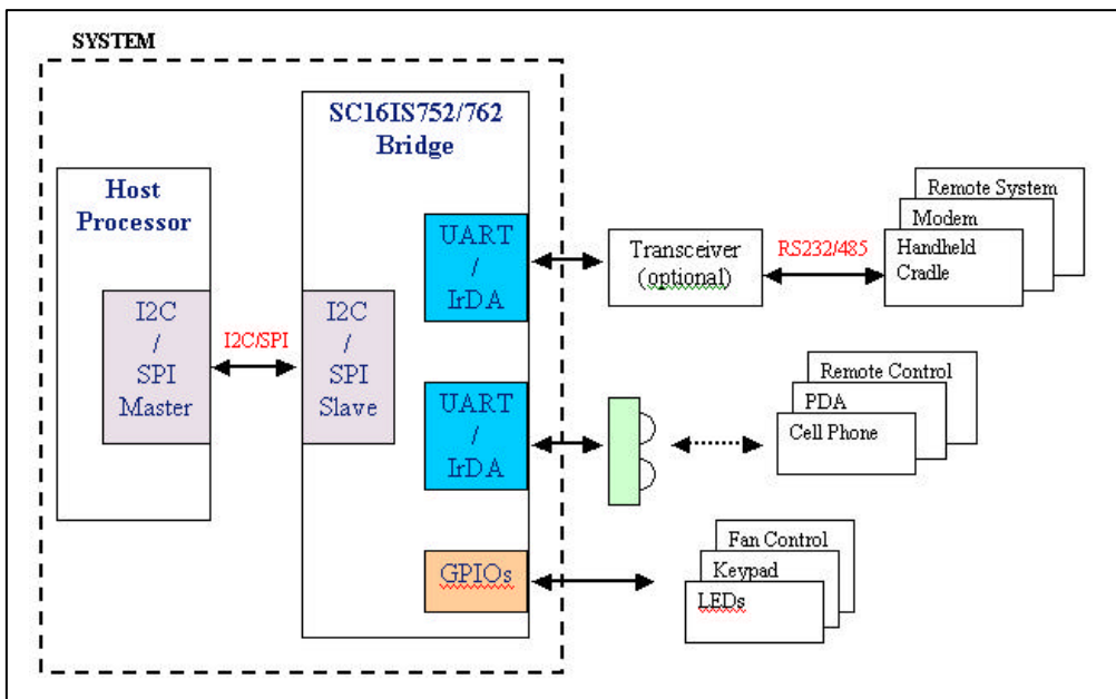
Figure 6. SC16IS752/762 Application Diagram
