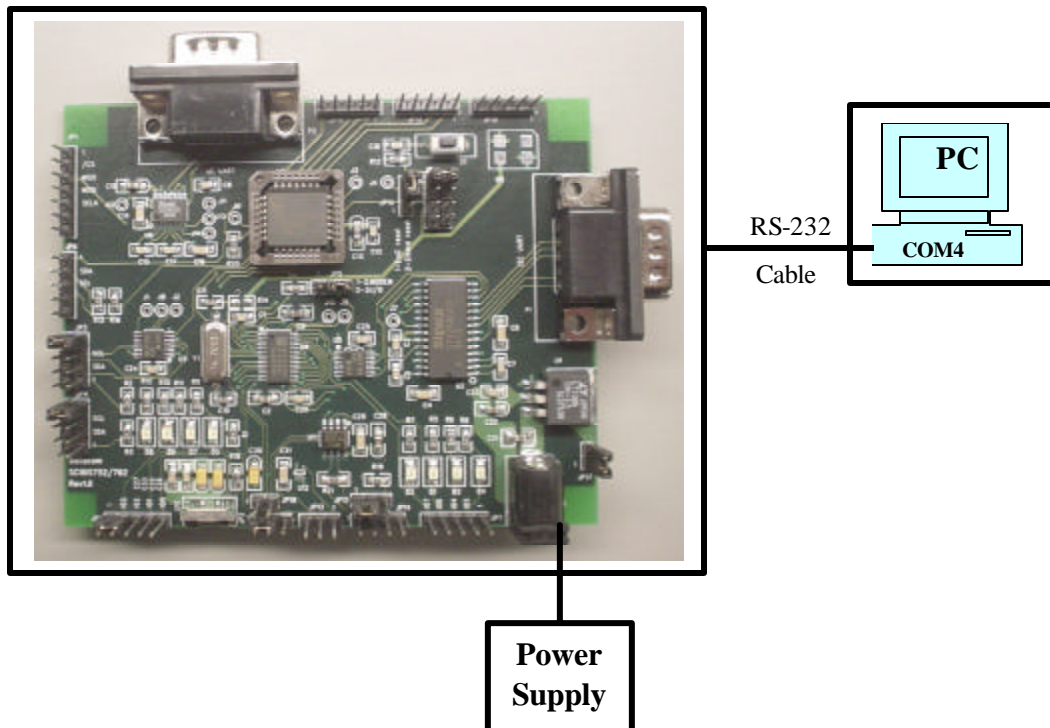
Figure 1. SC16IS752/762 Hardware Connection
