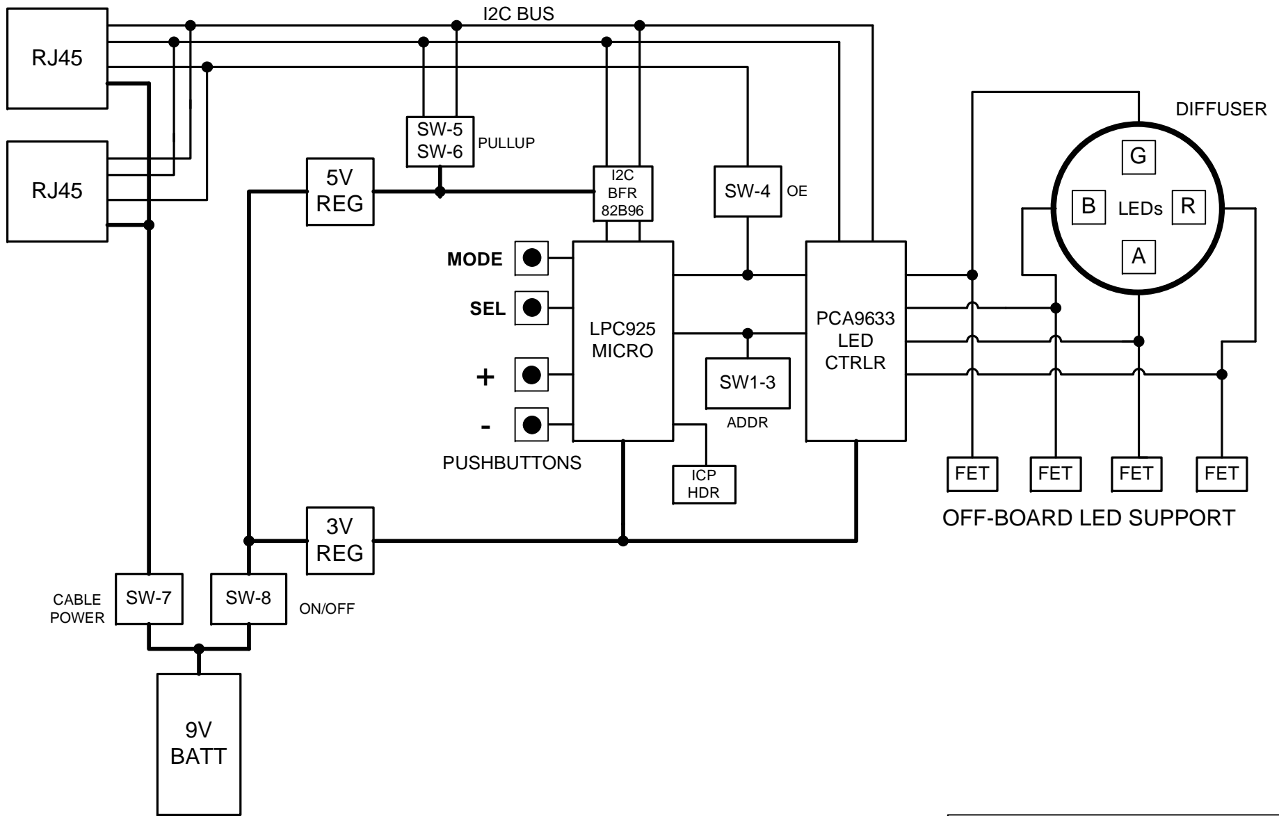
PCA9633 DEMO BLOCK DIAGRAM 5/4/2006 FUTURE DESIGNS, INC. www.teamfdi.com
