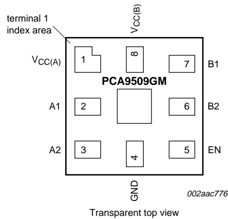
Fig 4. Pin configuration for XQFN8
