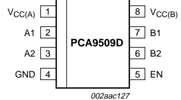
Fig 3. Pin configuration for SO8
