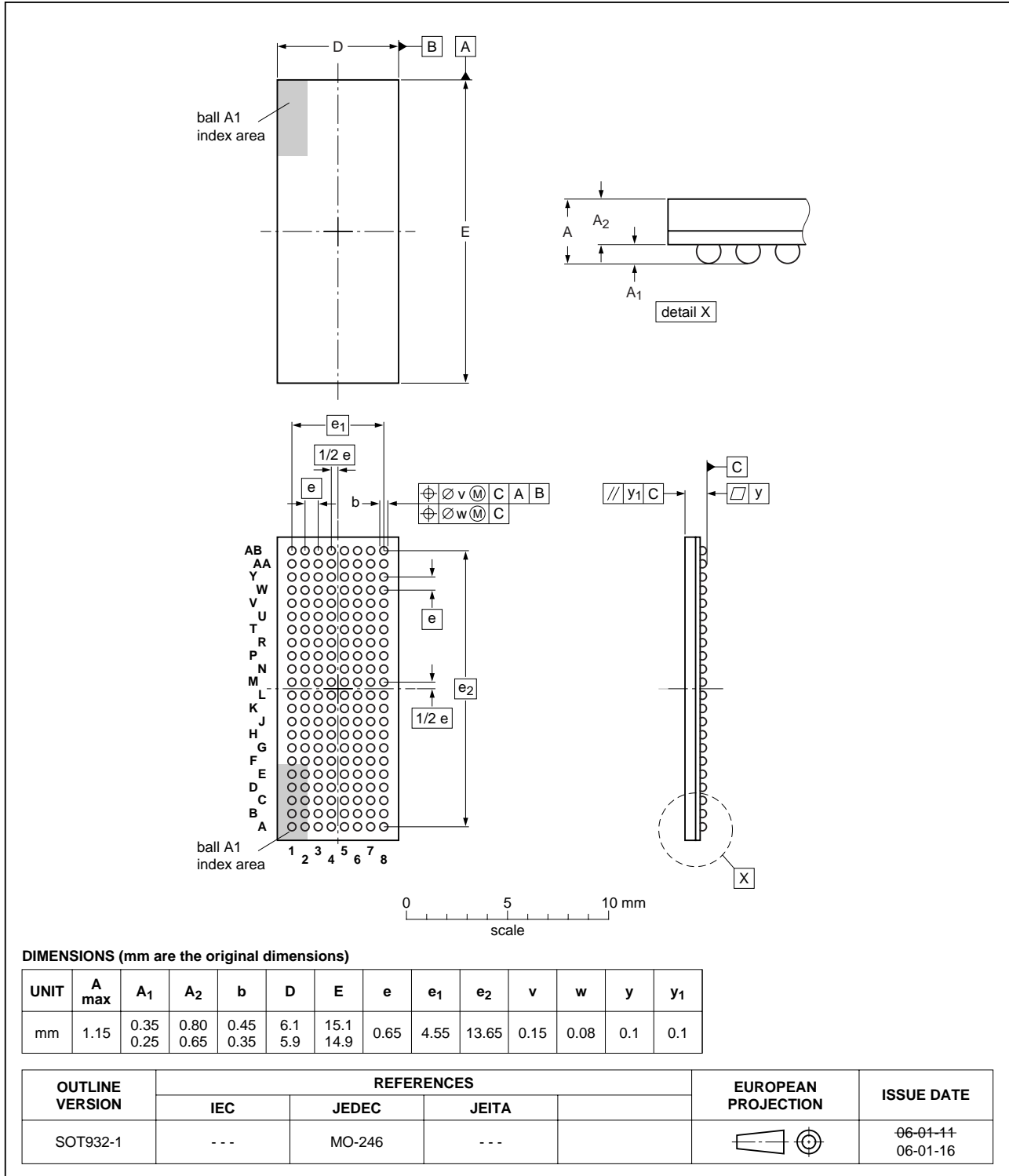
TFBGA176: plastic thin fine-pitch ball grid array package; 176 balls; body 6 x 15 x 0.7 mm
