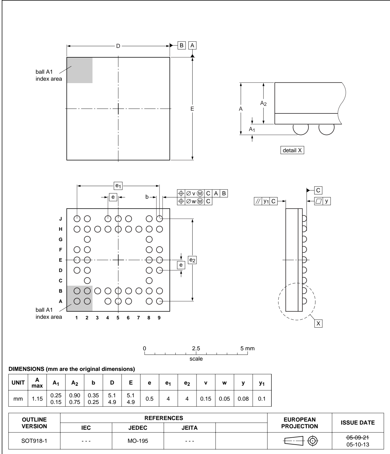
TFBGA48: plastic thin fine-pitch ball grid array package; 48 balls; body 5 x 5 x 0.8 mm
