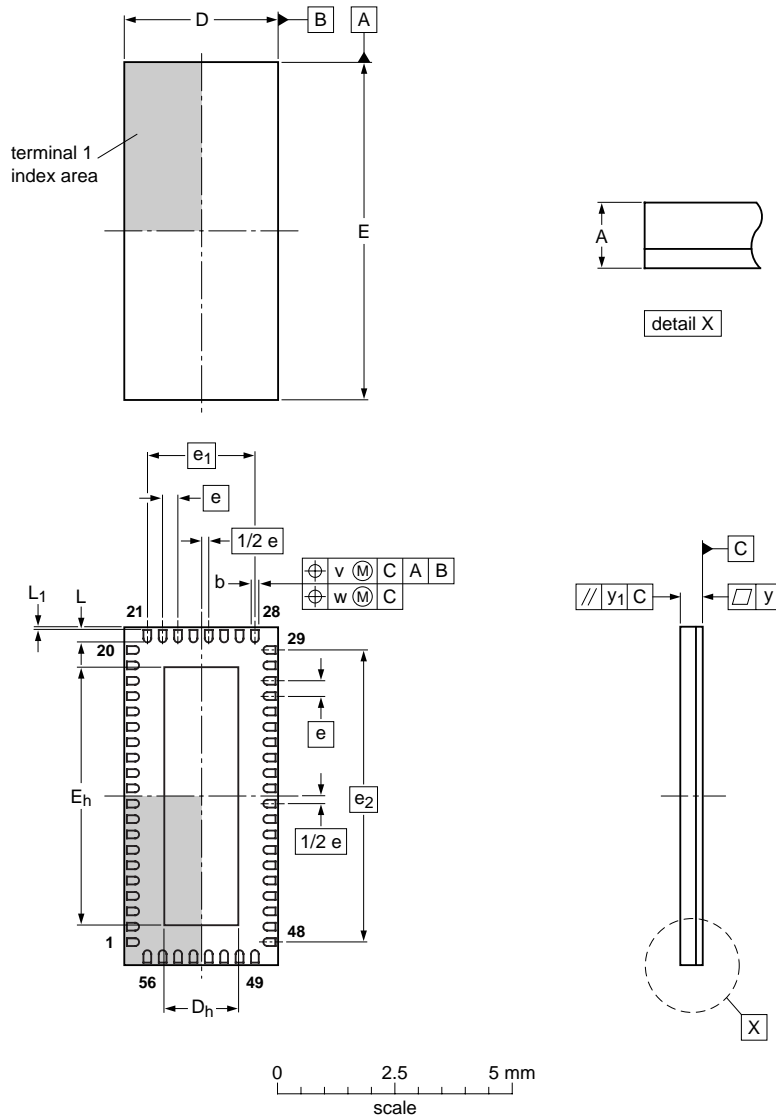
DIMENSIONS (mm are the original dimensions)
