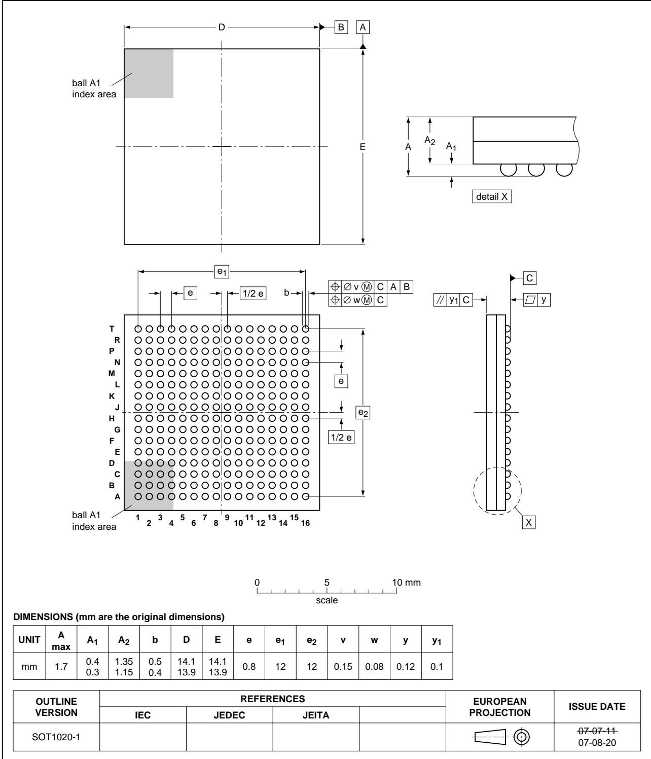
LFBGA256: plastic low profile fine-pitch ball grid array package; 256 balls
